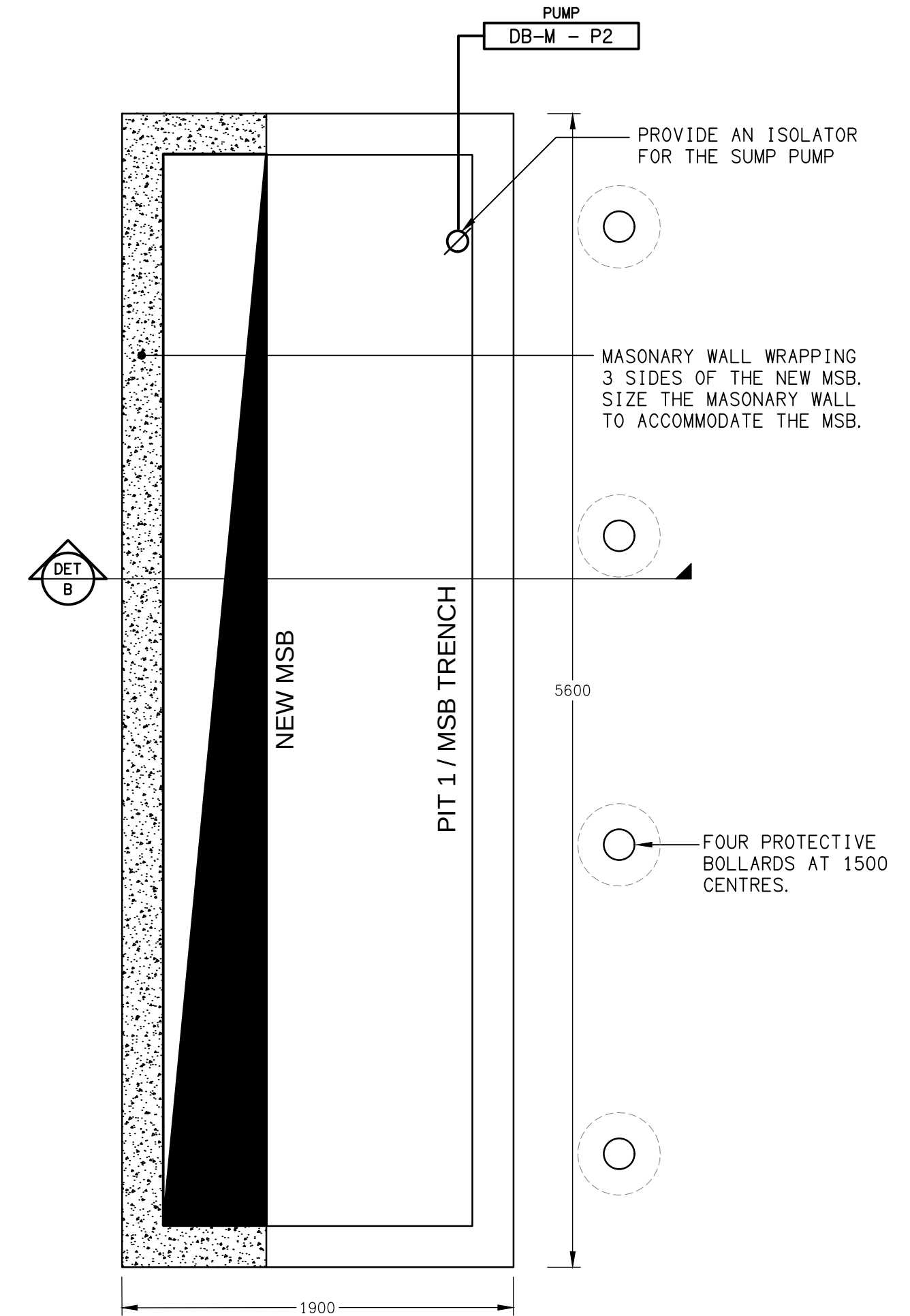
DETAIL A MSB / PIT 1 PLAN VIEW SCALE 1:25
