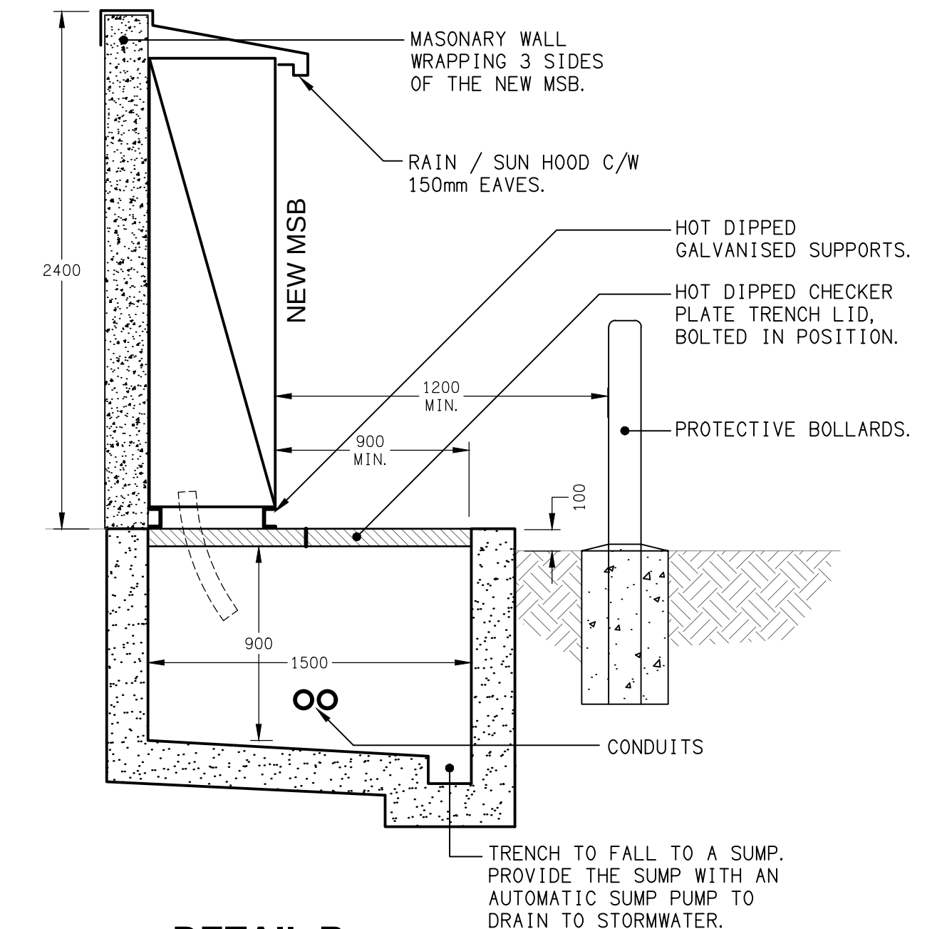
DETAIL B MSB / PIT 1 SECTION VIEW SCALE 1:25
