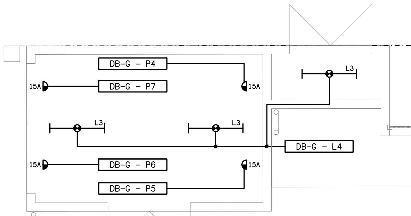
DETAIL C FIRE BOOSTER PLAN SCALE 1:50
